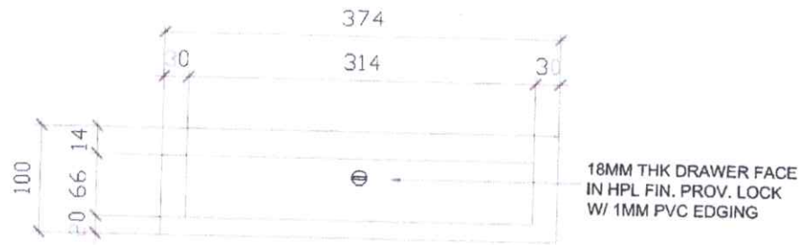
FRONT ELEV.
