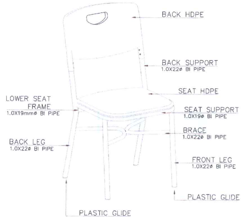
LEARNER'S CHAIR PERSPECTIVE VIEW
