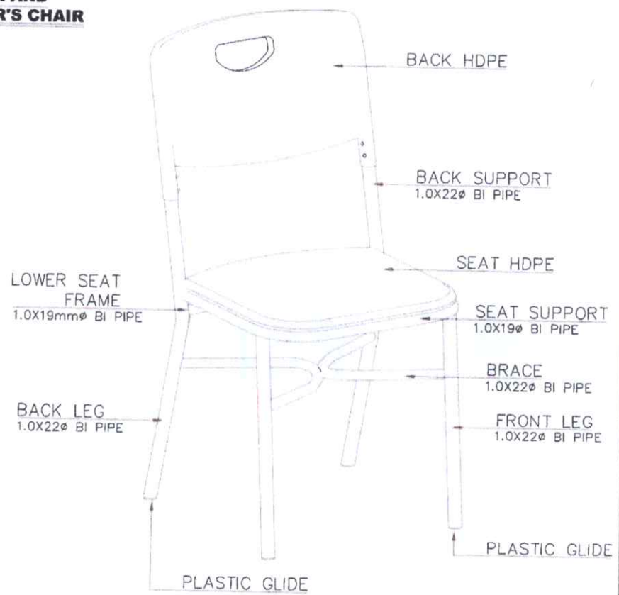
LEARNER'S CHAIR PERSPECTIVE VIEW
