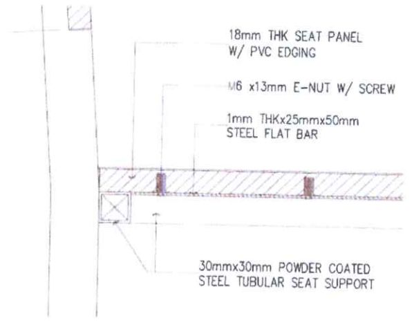
4 DETAIL - 2 3 SCALE 1 : 50 M
