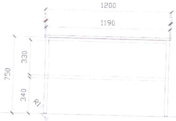
FRONT ELEV.
