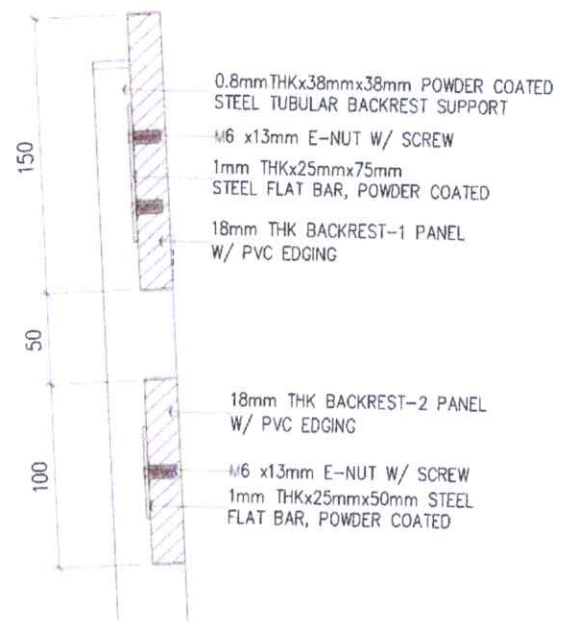
3 DETAIL - 1 3 SCALE 1 : 50 M
