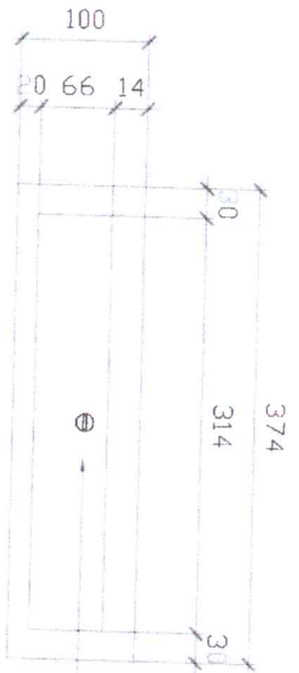
FRONT ELEV.
